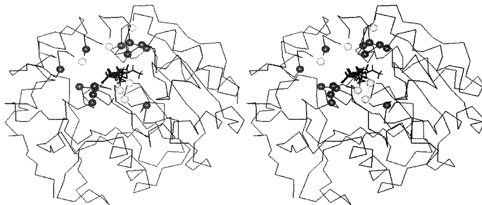
FIGURE 7: Stereoview of DhlA with assigned energy contributions. The protein backbone is represented by the \text{C}\alpha trace. The \text{C}\alpha atoms of the residues showing the most important energy contributions in model 4 are shown as balls (see Table 4). Dark-colored residues have only van der Waals energy contributions, while light-colored residues have both van der Waals and electrostatic energy contributions. The substrate molecules are in the positions obtained from energy minimization.
